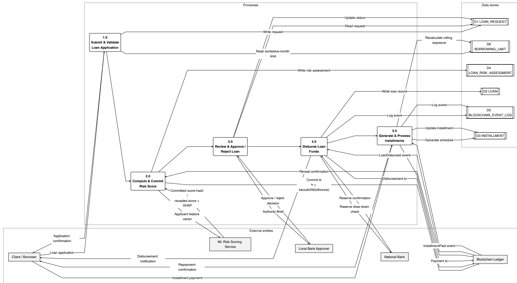
Figure 4.27: DFD Level 1.
