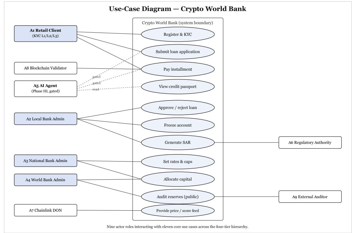
Figure 4.22: Use-case diagram.
