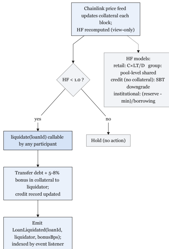
Figure 4.13: Liquidation engine.
