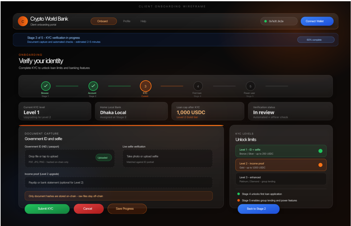
Figure 4.35: Onboarding wireframe.
